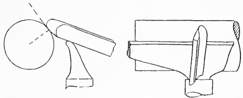
FIG. 291. CORRECT POSITION OF GOUGE IN ROUGHING OFF.
